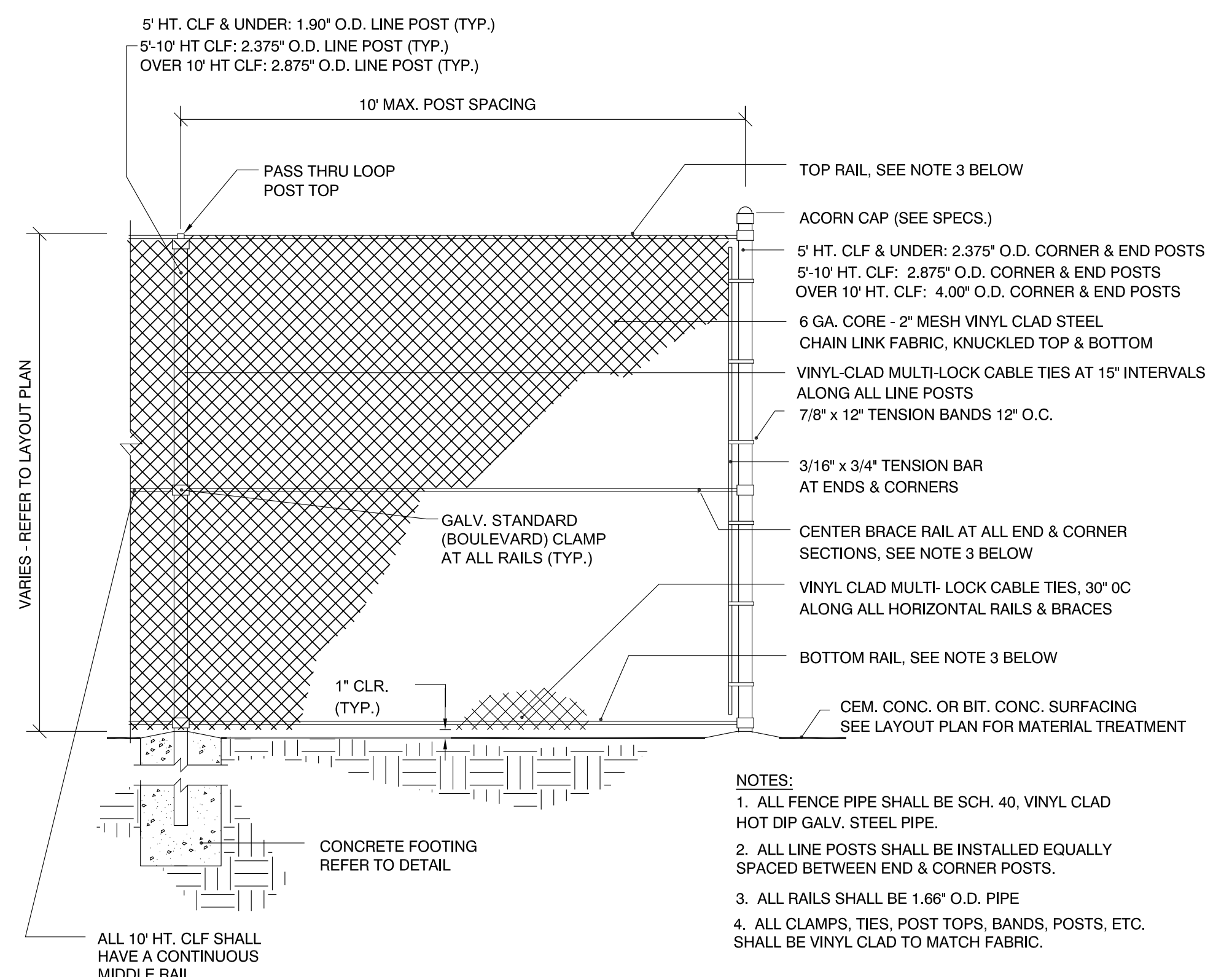
3 BLACK VINYL CLAD CHAIN LINK FENCE - 10' HT. OR LESS SCALE: N.T.S.
