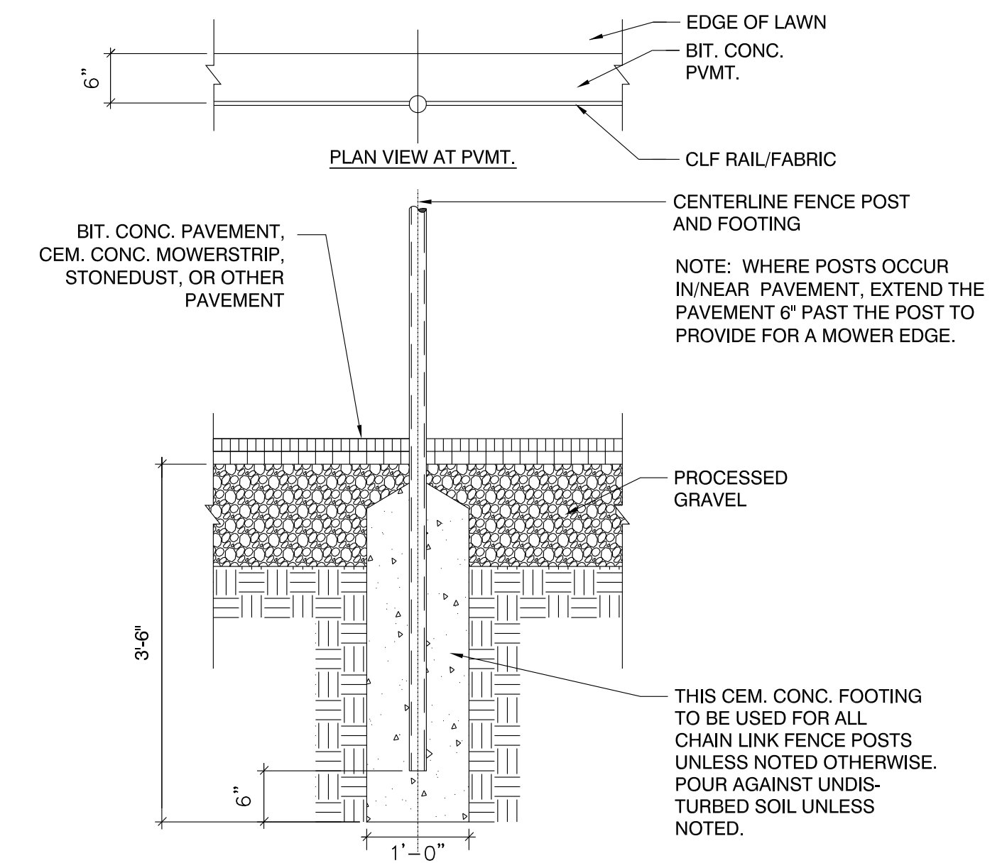
4 TYPICAL FENCE POST FOOTING SCALE: N.T.S.
